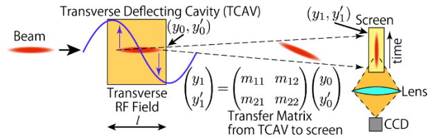
Figure 5: Schematic setup of a transverse deflector system.
