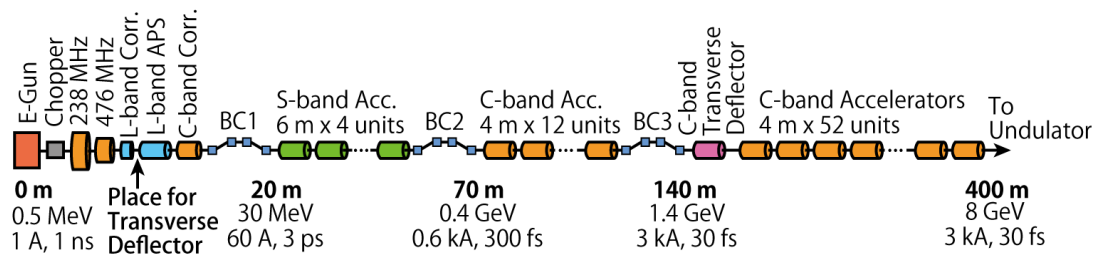
Figure 1: Schematic layout of the SACLA accelerator.
