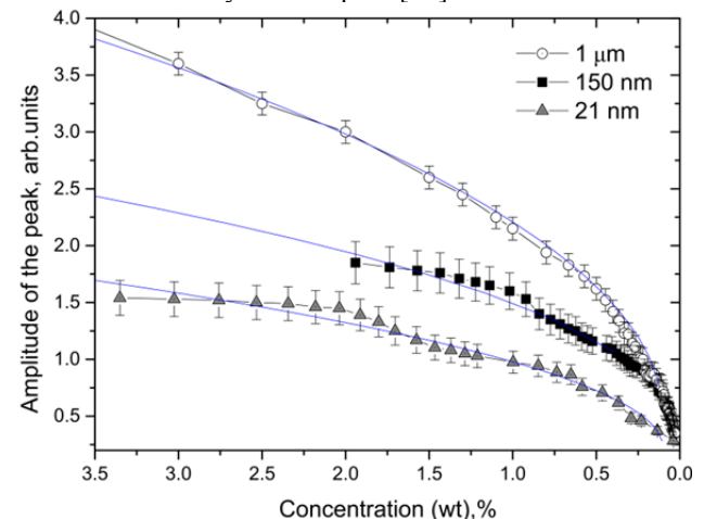
Figure 3: Measured influence of the concentration of TiO 2 seeders in water on the spectrum of the SM signal. Seeder diameter is indicated by different markers.
