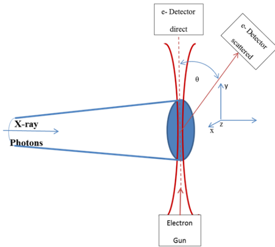
Figure 1: A high intensity x-ray beam from an FEL can be measured with a probe beam of low energy electrons by detecting the scattered electrons.
