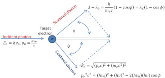
Figure 2: Compton scattering geometry for a photon scattered from a stationary electron.
