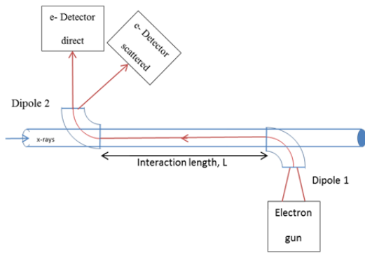
Figure 3: Back scatter geometry where the probe electron beam counter propagates over a length L against the x-ray beam.
